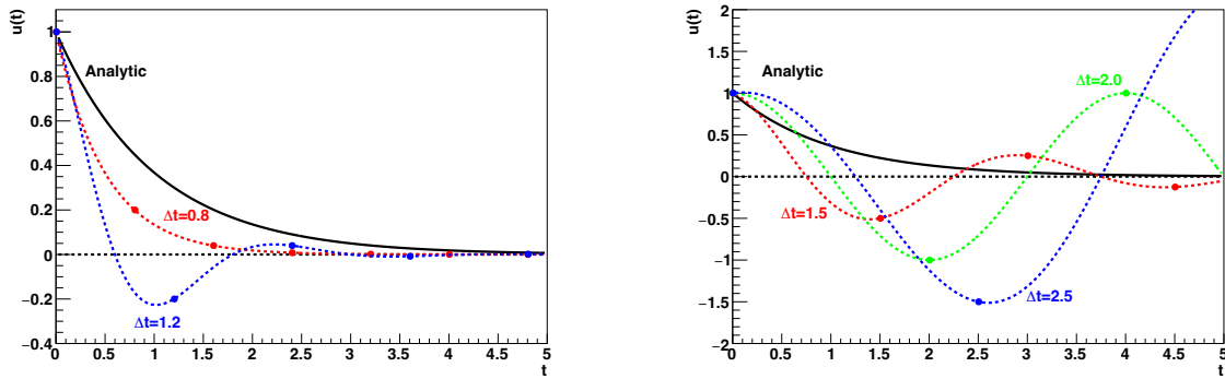
Figure 11.5: Left: First few steps for the Euler method with a = -1 compared with the analytic solution (black), for \Delta t = 0.8 (red) and 1.2 (blue). The dashed lines show the analytic modified differential equation solutions which the Euler step values obey. Right: The same as the left plot but for \Delta t = 1.5 (red), 2.0 (green) and 2.5 (blue).
